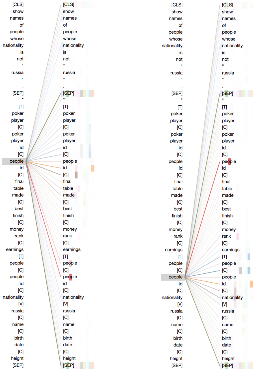
Figure A6: Visualization of attention in layer 5 between a pair of foreign keys.
